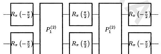
FIG. 1. Gate sequence of Grover search on two qubits.
